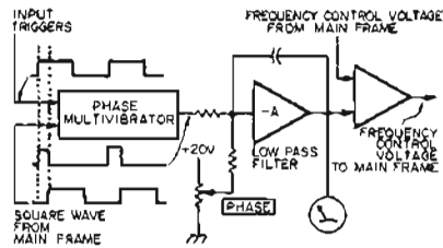
Figure 3. Block diagram of 3302A plug-in phase lock mode.
