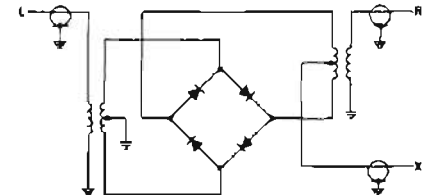
Figure 2. Schematic diagram
