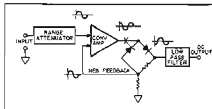
Figure 7. Typical ac/dc converter.
