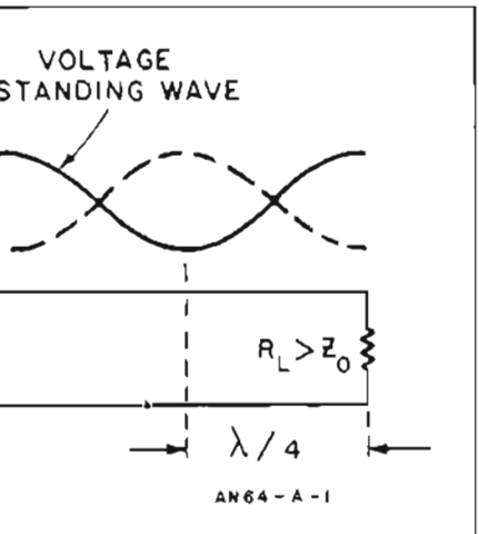
Figure 1. Mismatched transmission line exhibits standing waves, making voltage or current measurements arbitrary. At microwave frequencies, energy levels are more readily determined by power measurement which is independent of position (lossless line).
