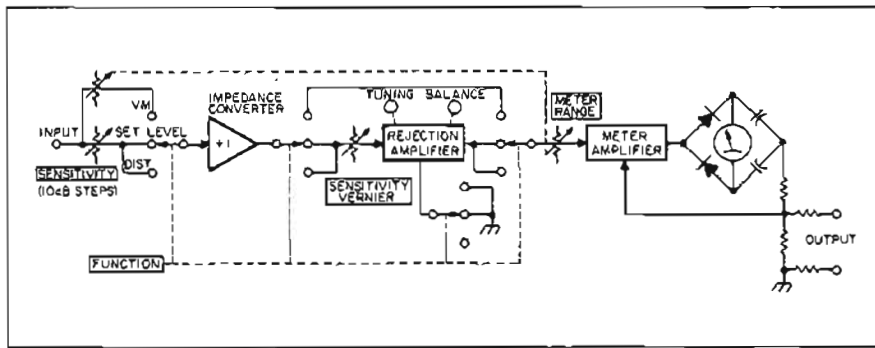
Figure 3. Elements of Distortion Analyzer Instrument function as broadband calibrated ac voltmeter in 'Voltmeter' mode and as signal-level indicator in 'Set Level' mode. In 'Distortion' mode, Rejection Amplifier can be tuned to suppress fundamental frequency of input signal, permitting comparison of distortion component's level to total signal level.
